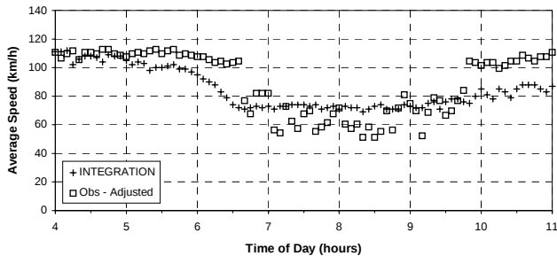
Fig. 10: Average 5 minute simulated and normalised observed speeds for detector station 7
